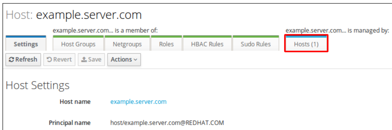
Figure 18.2. Host Subtab
