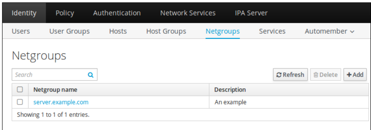
Figure 23.1. Netgroups List
