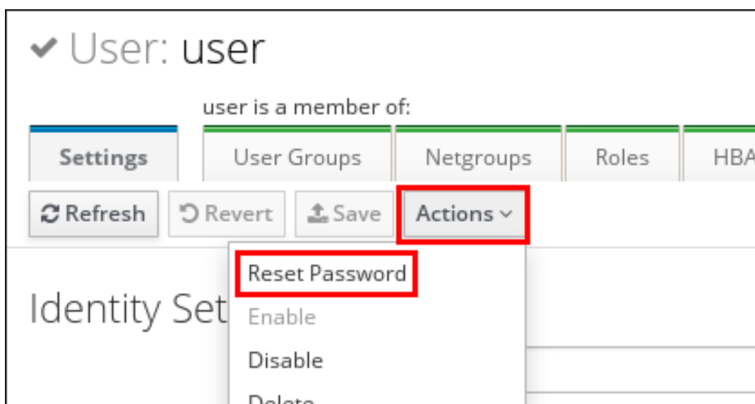
Figure 11.2. Resetting Password
