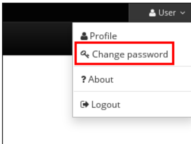
Figure 11.1. Resetting Password
