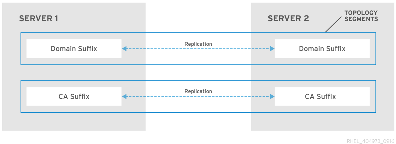
Figure 6.2. Topology Segments
