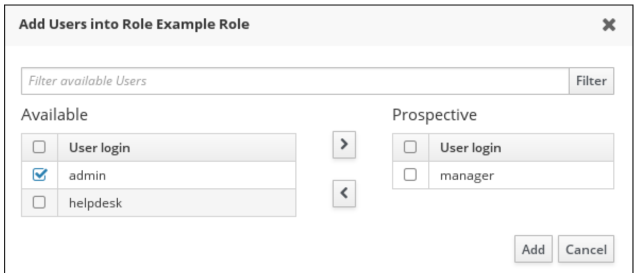
Figure 31.9. Selecting Users
