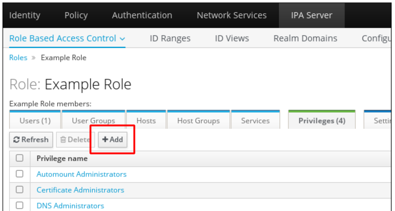
Figure 31.10. Adding Privileges
