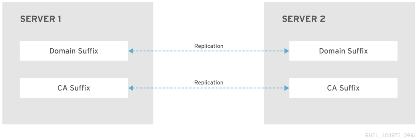
Figure 6.1. Topology Suffixes
