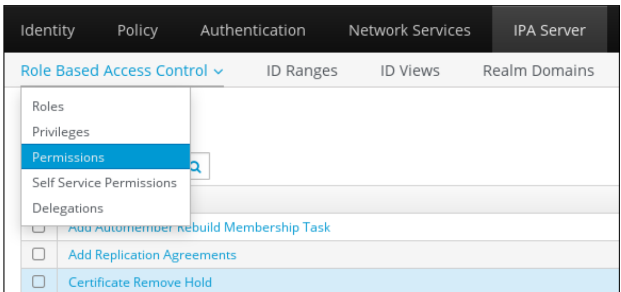
Figure 31.12. Permissions Task
