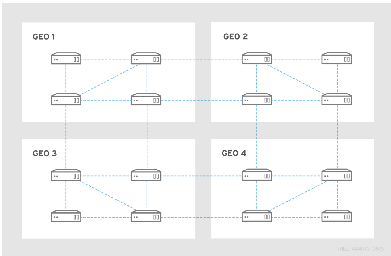
Figure 4.5. Topology Example
