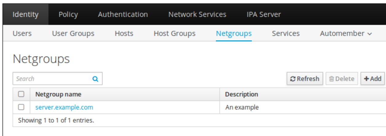
Figure 23.4. Netgroups List
